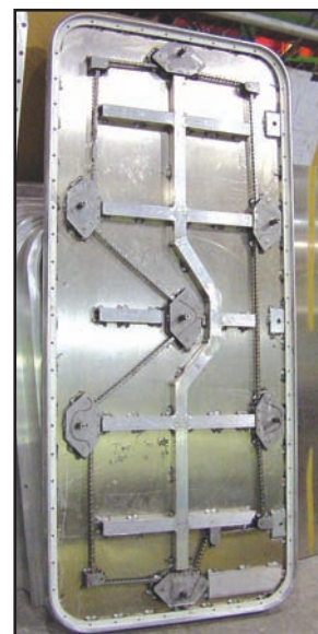
Chain-drive, Stiffeners, Interior panel with inspection plate at left in photo
